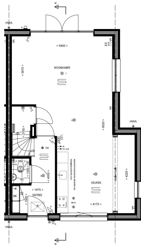
Begane grond 1:50 Bnr: 19 Type: A4
