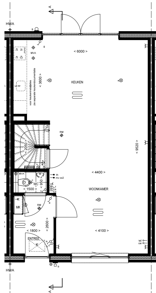
Begane grond 1:50 Bnr: 30 Type: C7
