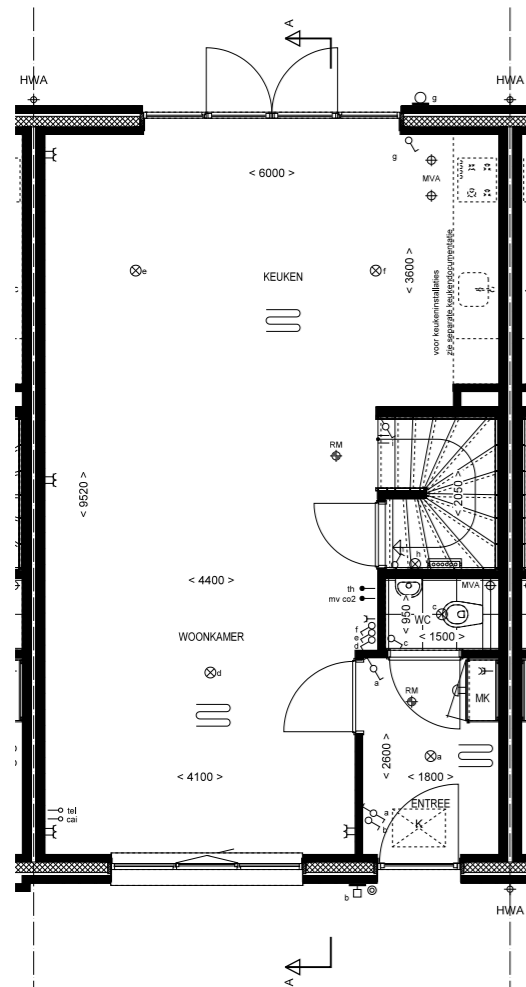
Begane grond 1:50 Bnr: 31 Type: C7sp
