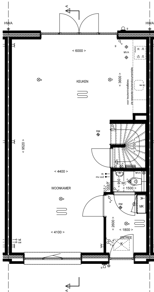
Begane grond 1:50 Bnr: 32 Type: C8sp
