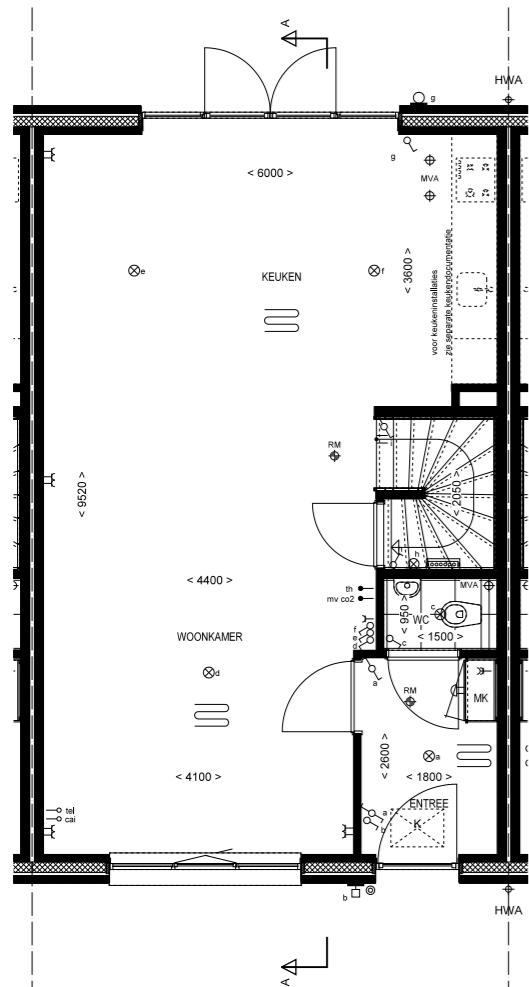
Begane grond 1:50 Bnr: 34 Type: C7sp
